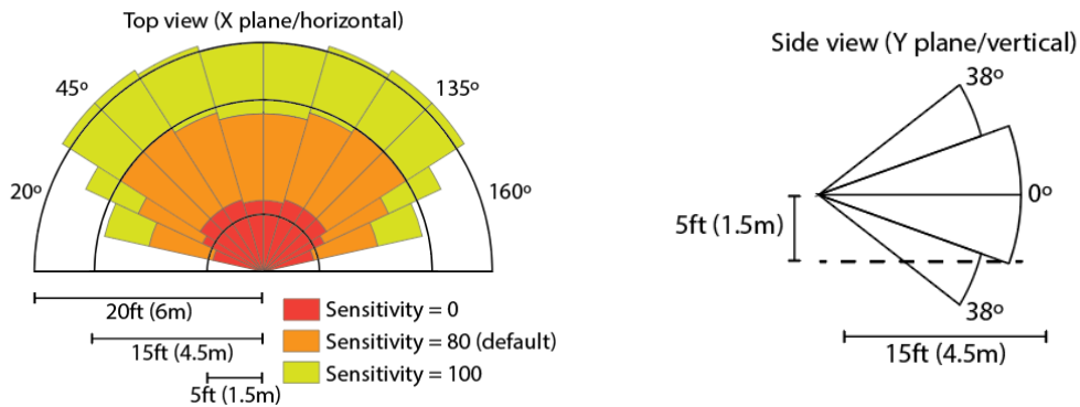
Figure 3: PIR Sensitivity
